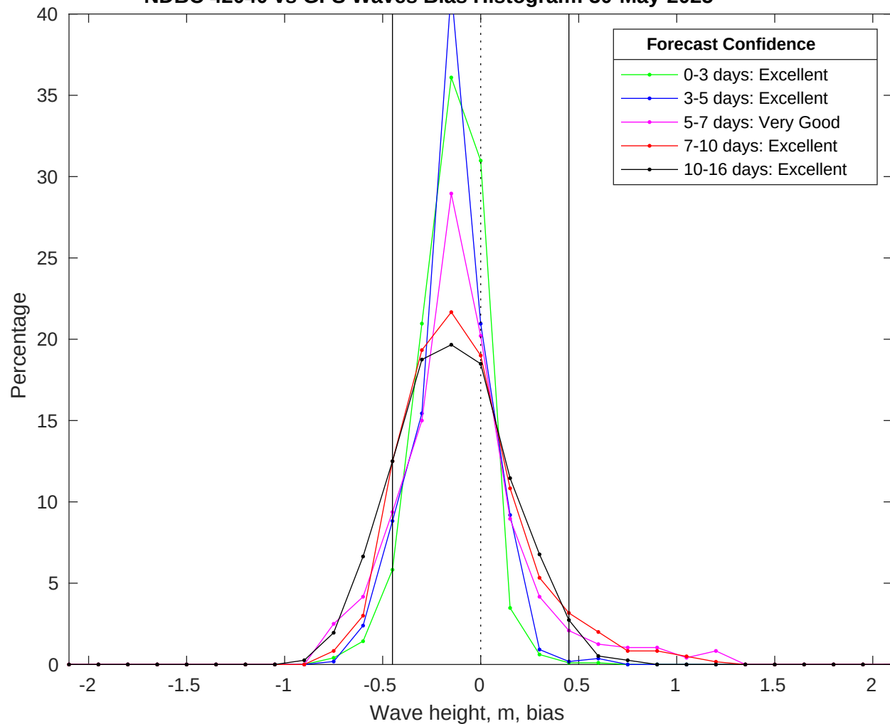
NDBC 42040 vs GFS Waves Bias Histogram: 30-May-2025
