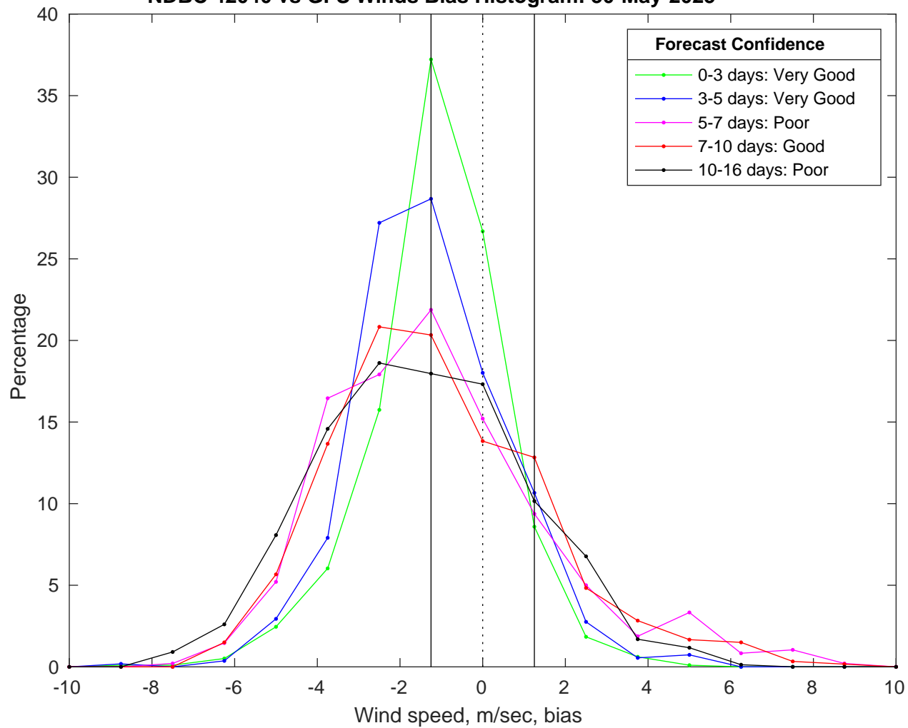
NDBC 42040 vs GFS Winds Bias Histogram: 30-May-2025
