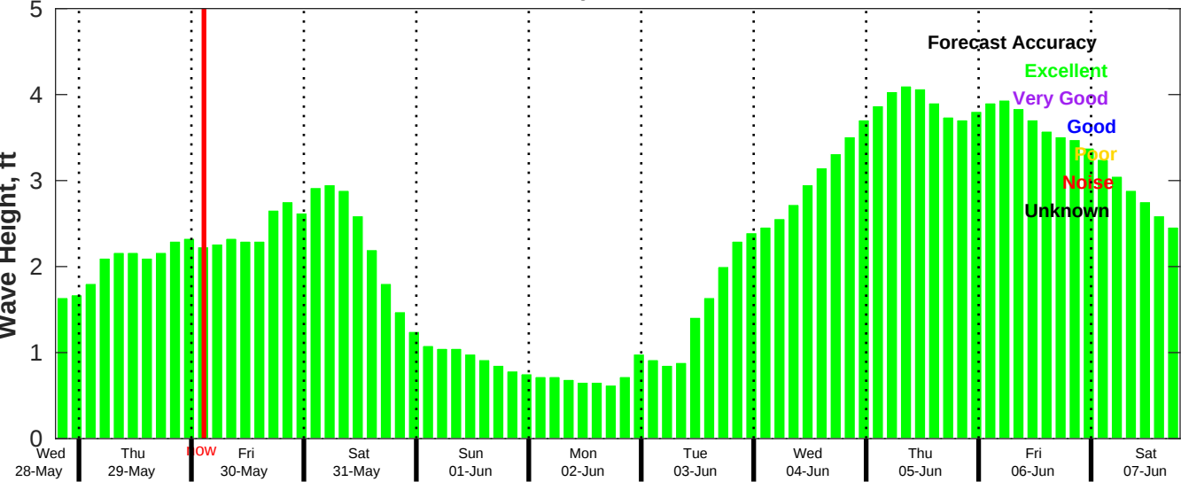
CMEMS Wave Forecast for NDBC 42040 from 28-May-2025 19:00:00 to 07-Jun-2025 19:00:00
