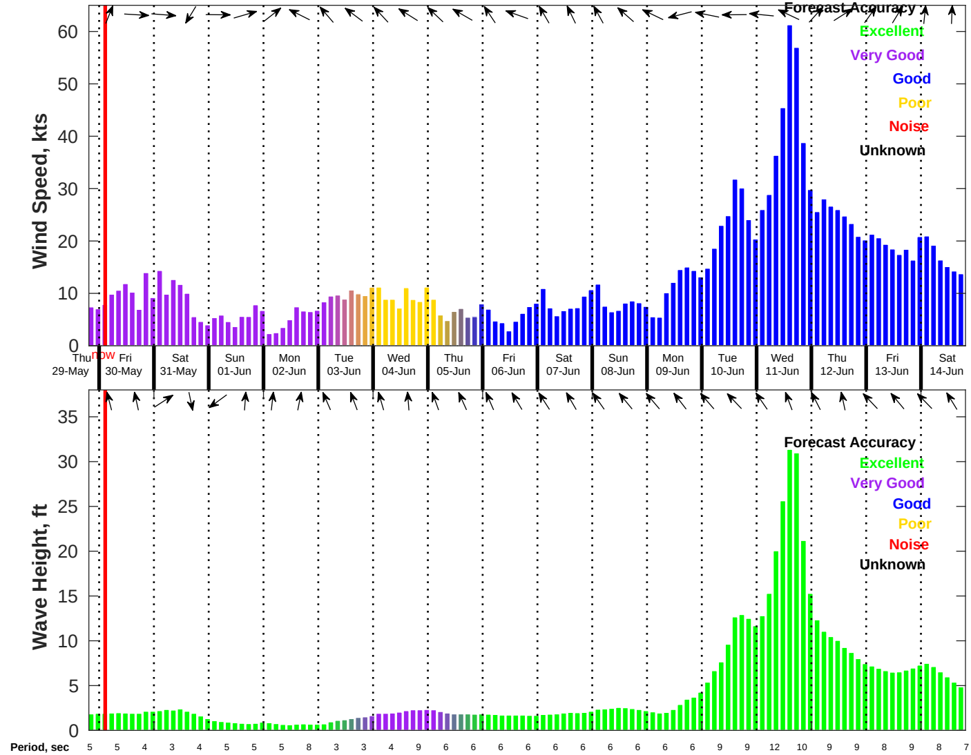
Wind & Wave Forecast for NDBC 42040 from 29-May-2025 19:00:00 to 14-Jun-2025 19:00:00
