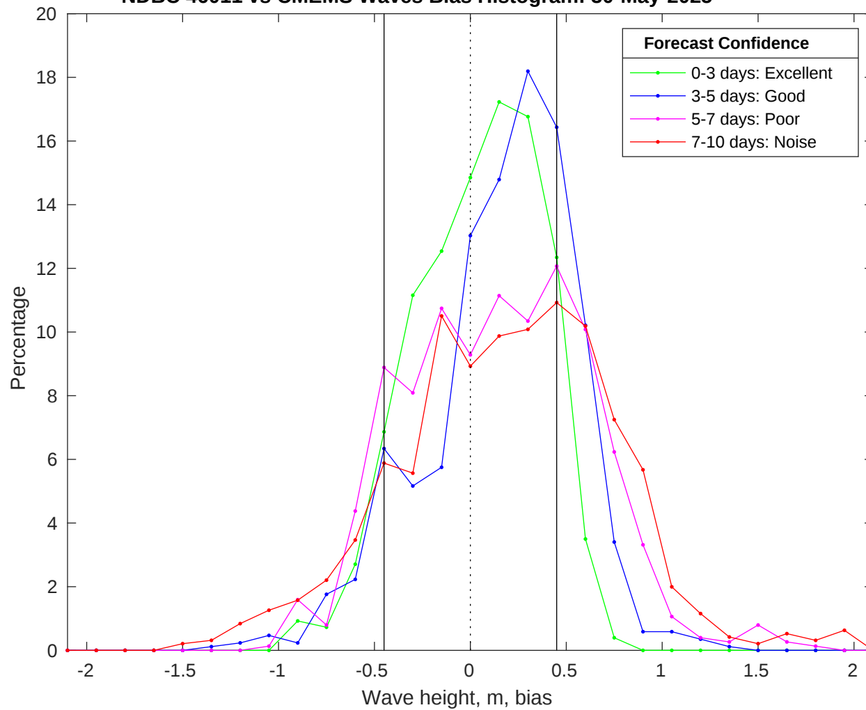
NDBC 46011 vs CMEMS Waves Bias Histogram: 30-May-2025
