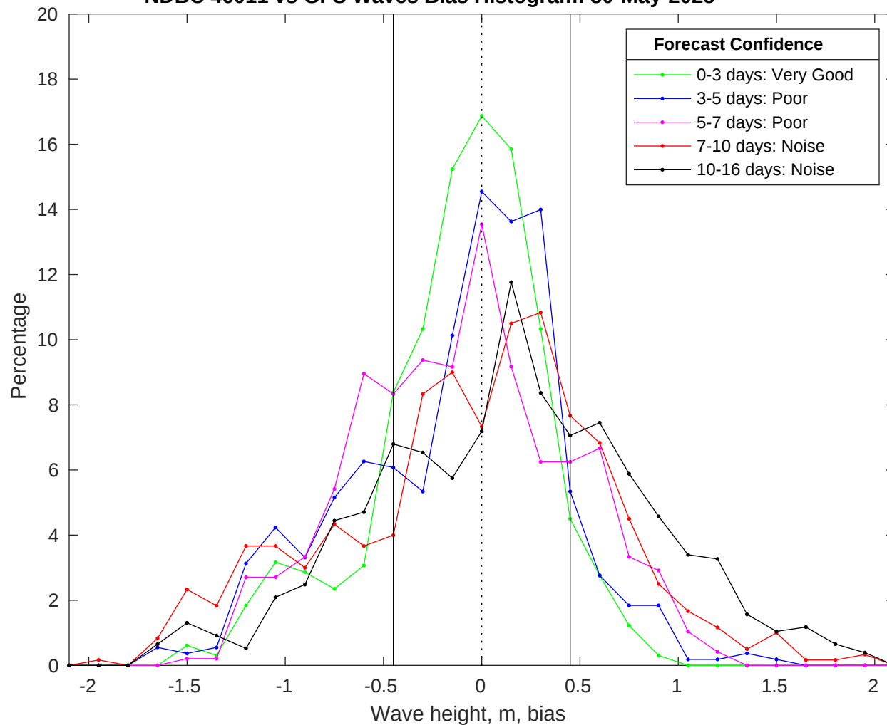
NDBC 46011 vs GFS Waves Bias Histogram: 30-May-2025
