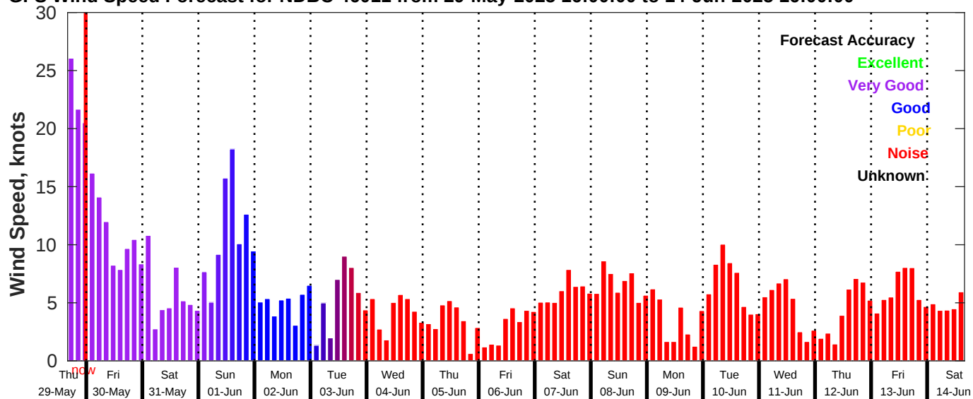
GFS Wind Speed Forecast for NDBC 46011 from 29-May-2025 16:00:00 to 14-Jun-2025 16:00:00
