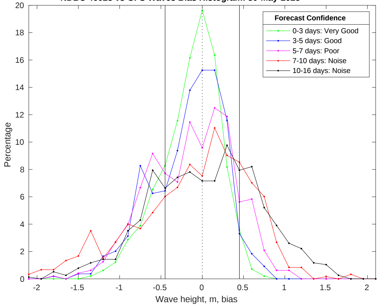
NDBC 46028 vs GFS Waves Bias Histogram: 30-May-2025
