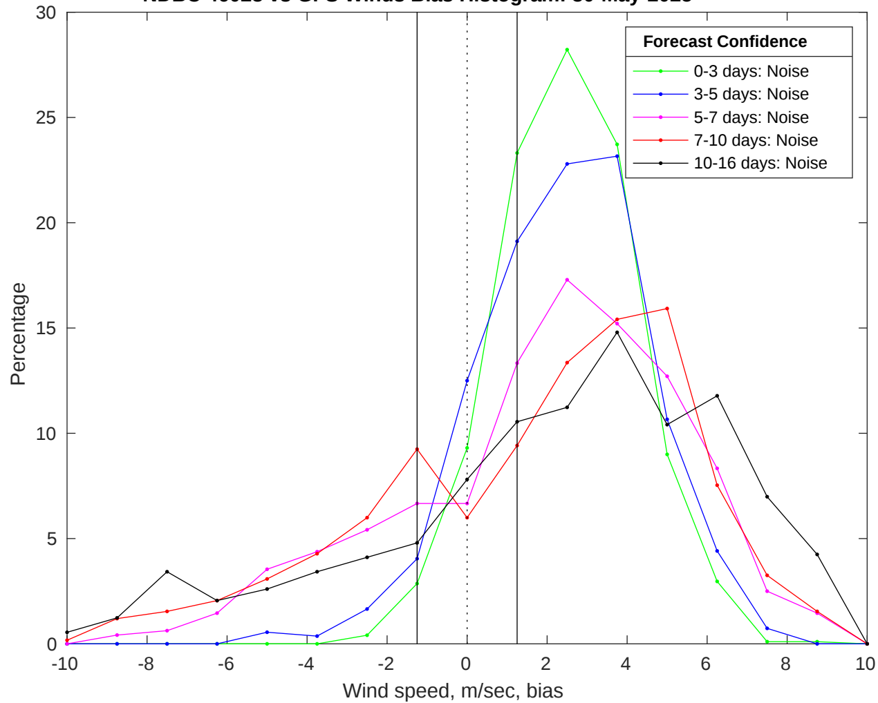
NDBC 46028 vs GFS Winds Bias Histogram: 30-May-2025
