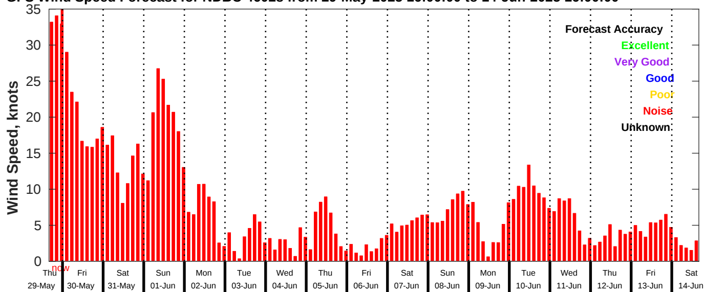
GFS Wind Speed Forecast for NDBC 46028 from 29-May-2025 16:00:00 to 14-Jun-2025 16:00:00
