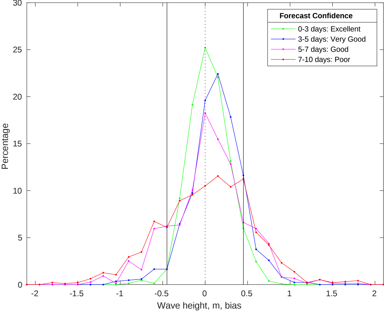
NDBC 46054 vs CMEMS Waves Bias Histogram: 30-May-2025
