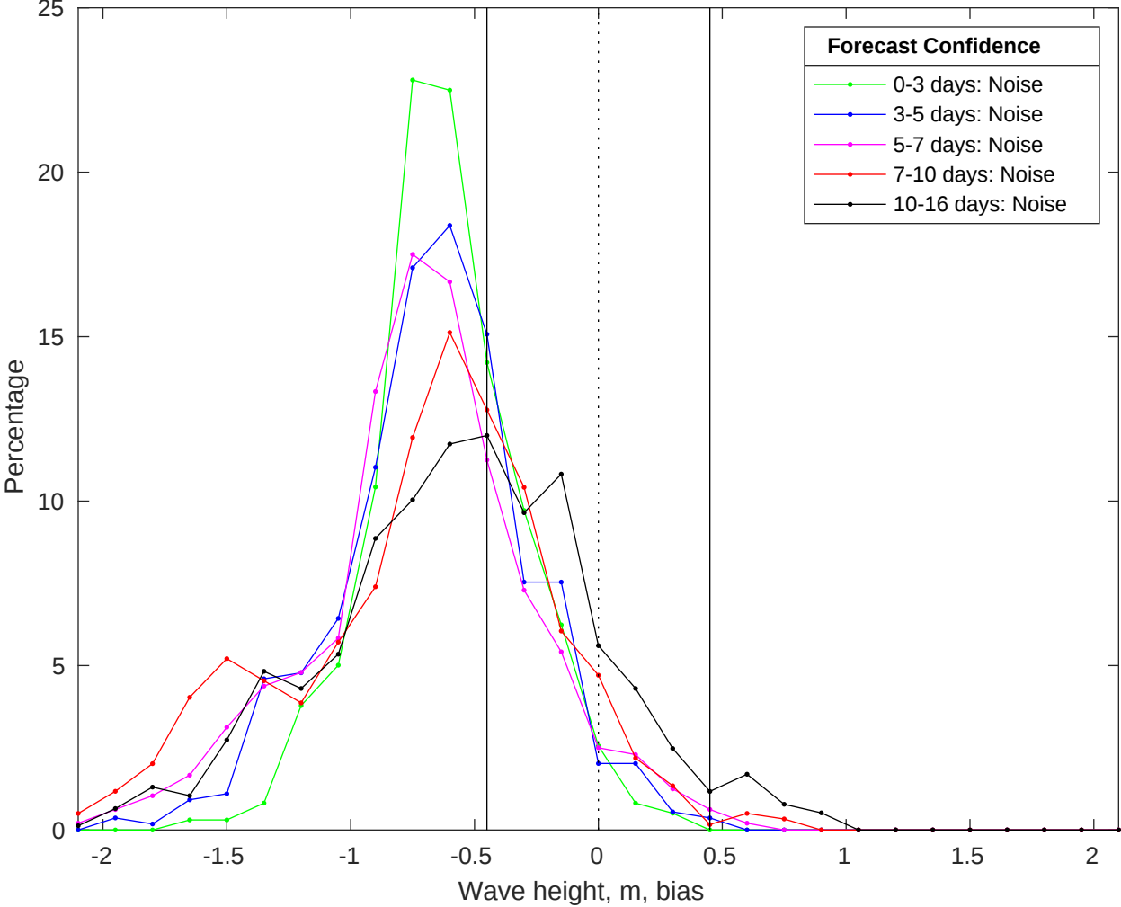
NDBC 46054 vs GFS Waves Bias Histogram: 30-May-2025
