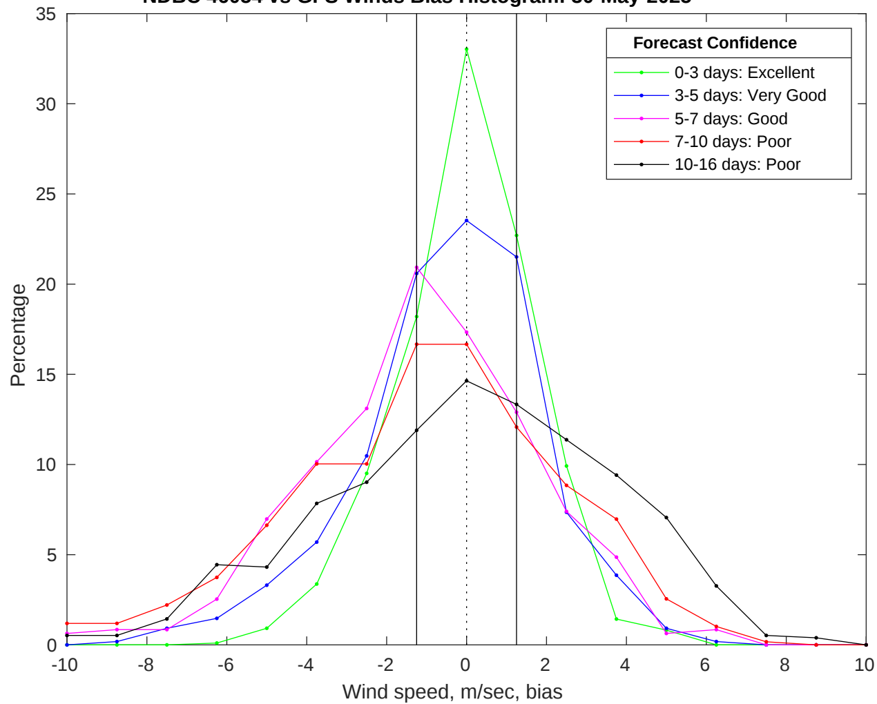
NDBC 46054 vs GFS Winds Bias Histogram: 30-May-2025
