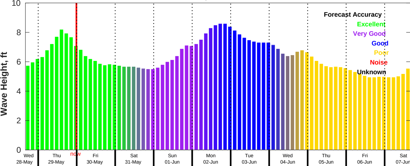
CMEMS Wave Forecast for NDBC 46054 from 28-May-2025 16:00:00 to 07-Jun-2025 16:00:00
