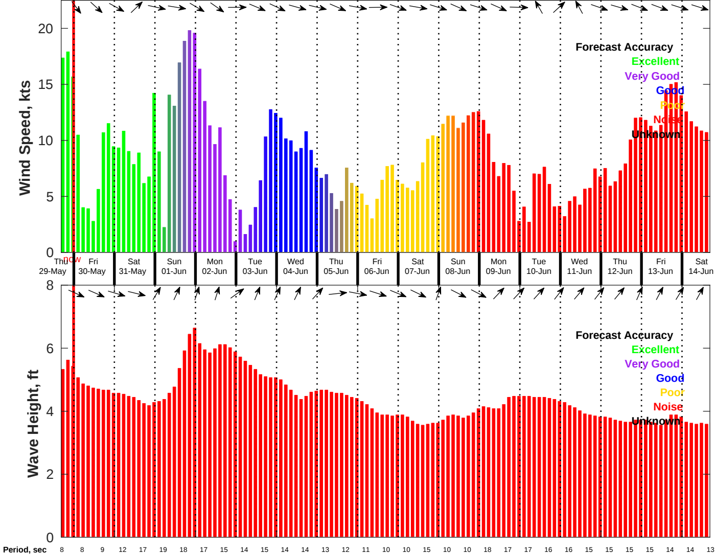
Wind & Wave Forecast for NDBC 46069 from 29-May-2025 16:00:00 to 14-Jun-2025 16:00:00
