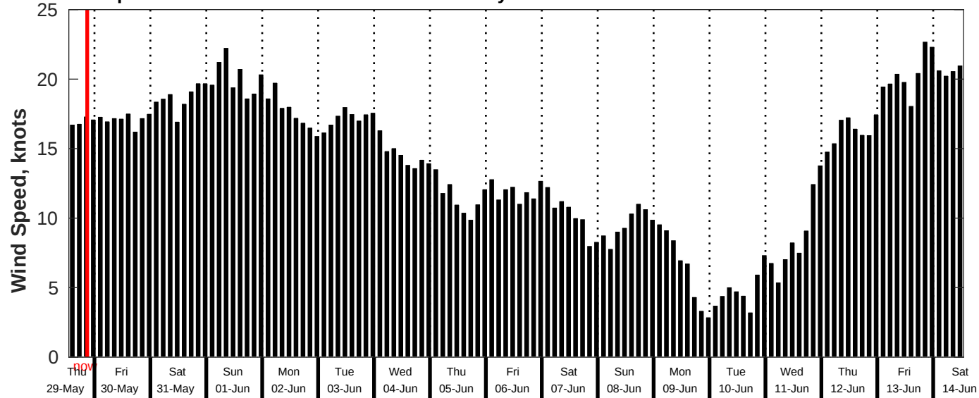
GFS Wind Speed Forecast for NDBC 51209 from 29-May-2025 13:00:00 to 14-Jun-2025 13:00:00
