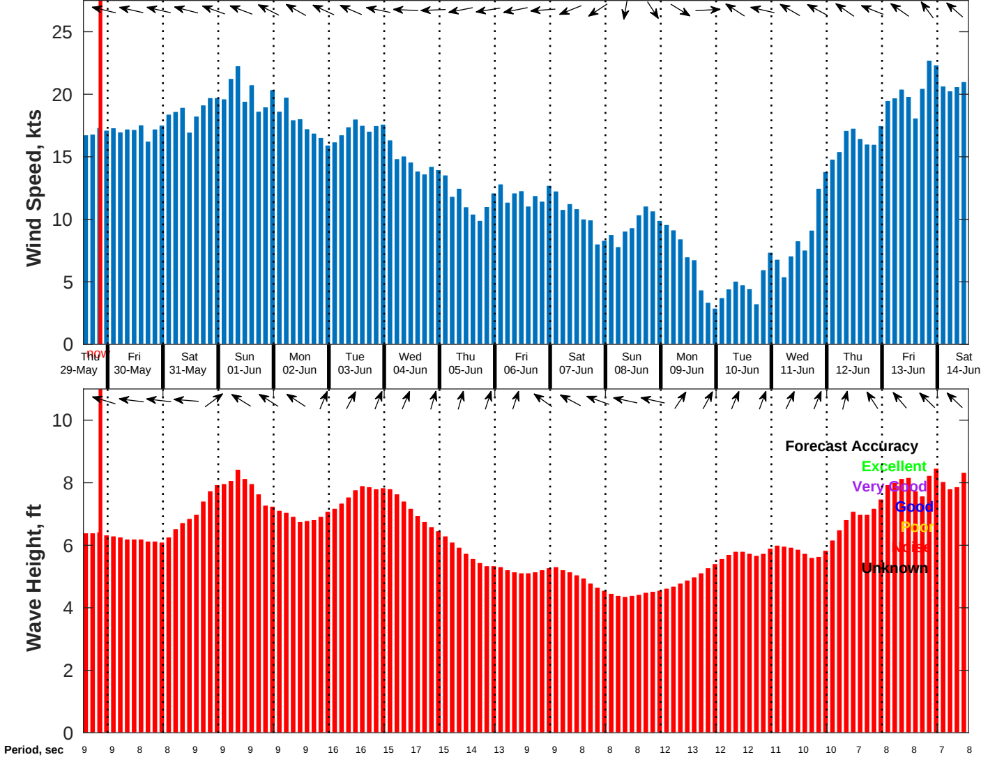
Wind & Wave Forecast for NDBC 51209 from 29-May-2025 13:00:00 to 14-Jun-2025 13:00:00
