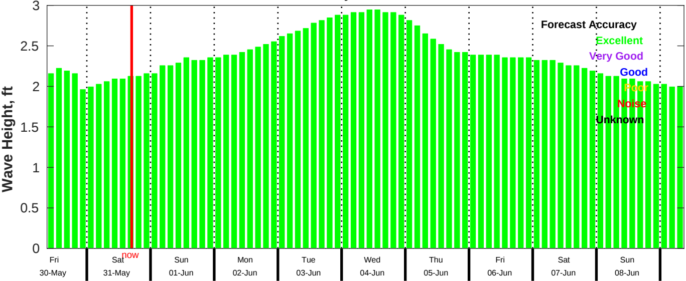
CMEMS Wave Forecast for NDBC 52212 from 29-May-2025 09:00:00 to 08-Jun-2025 09:00:00
