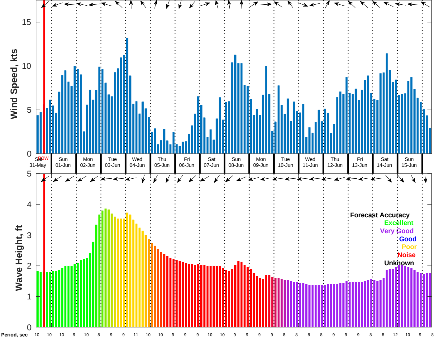
Wind & Wave Forecast for NDBC 52212 from 30-May-2025 09:00:00 to 15-Jun-2025 09:00:00
