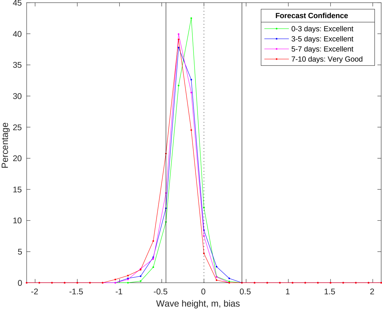
NDBC 52213 vs CMEMS Waves Bias Histogram: 30-May-2025
