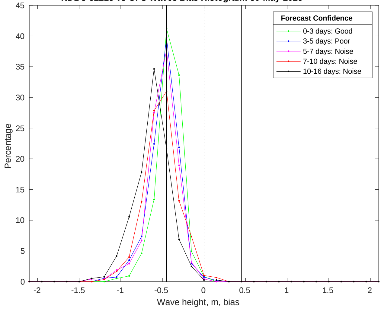
NDBC 52213 vs GFS Waves Bias Histogram: 30-May-2025
