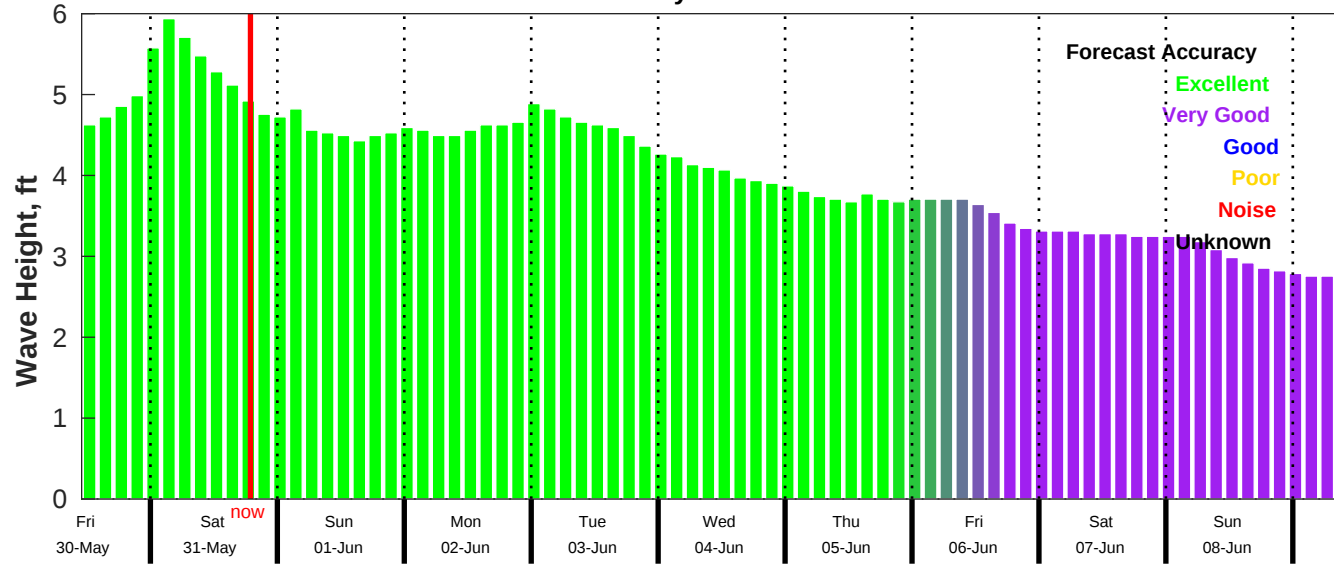
CMEMS Wave Forecast for NDBC 52213 from 29-May-2025 11:00:00 to 08-Jun-2025 11:00:00
