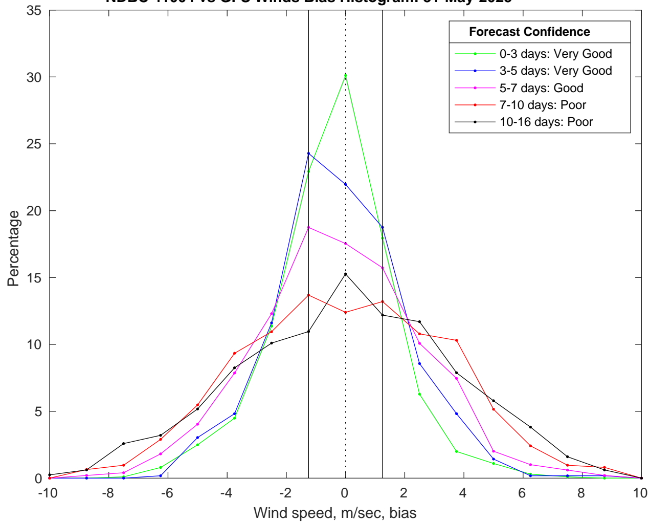
NDBC 41004 vs GFS Winds Bias Histogram: 31-May-2025
