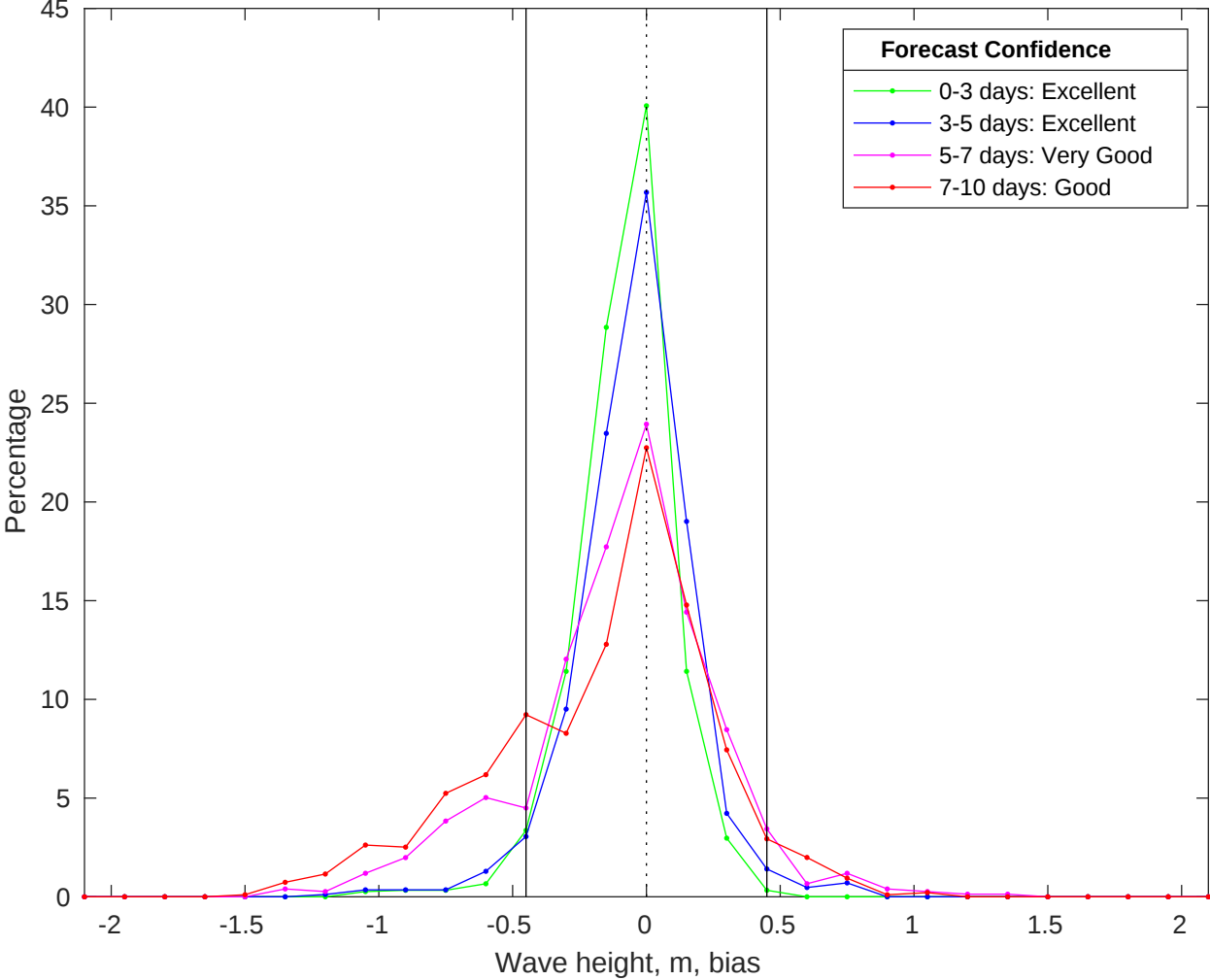
NDBC 41013 vs CMEMS Waves Bias Histogram: 31-May-2025
