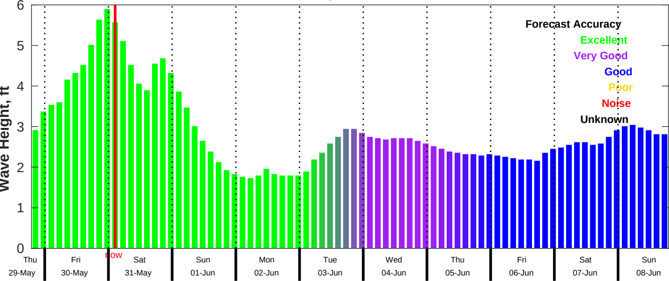
CMEMS Wave Forecast for NDBC 41013 from 29-May-2025 19:00:00 to 08-Jun-2025 19:00:00
