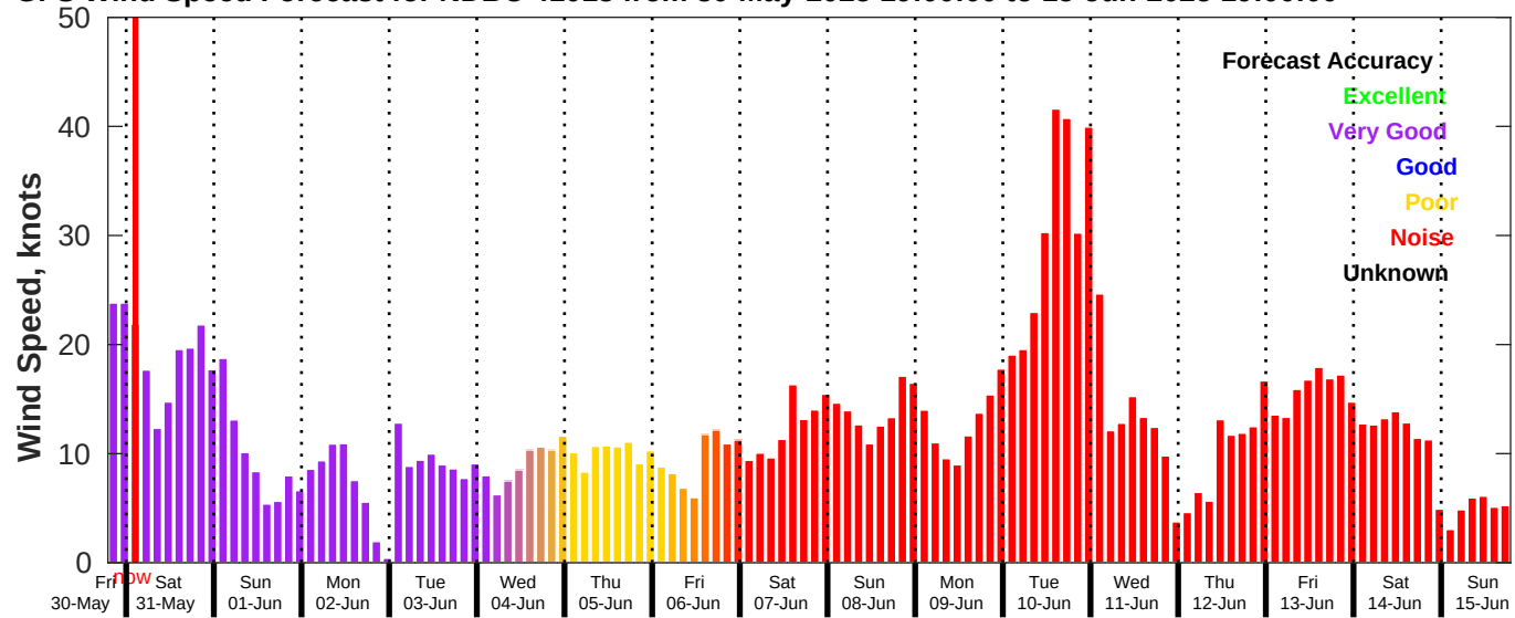
GFS Wind Speed Forecast for NDBC 41013 from 30-May-2025 19:00:00 to 15-Jun-2025 19:00:00
