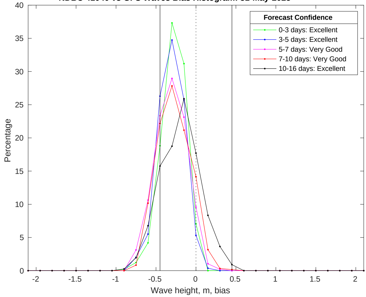
NDBC 41040 vs GFS Waves Bias Histogram: 31-May-2025
