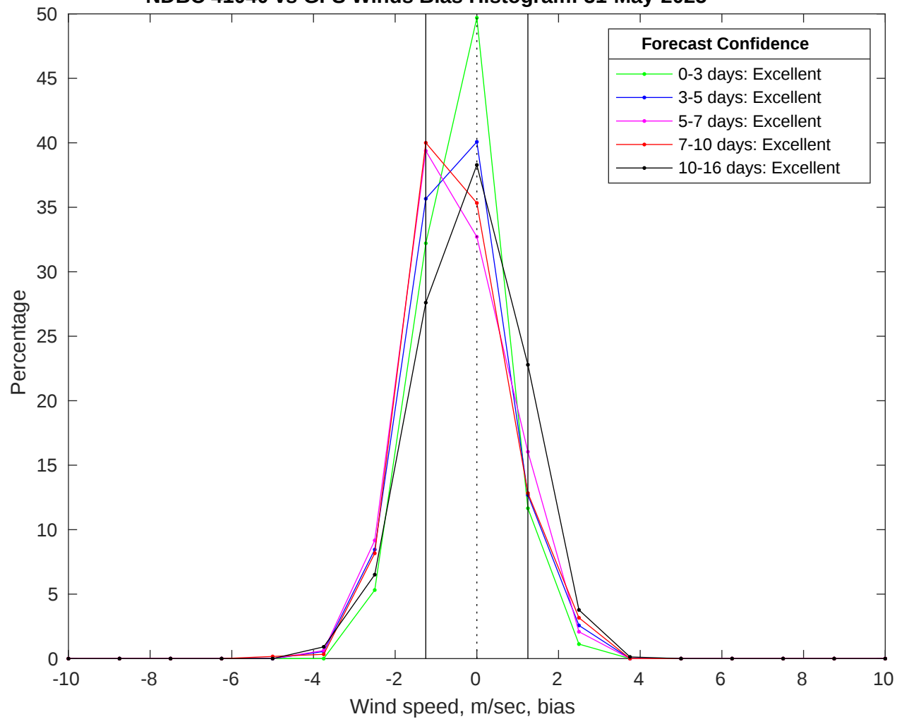
NDBC 41040 vs GFS Winds Bias Histogram: 31-May-2025
