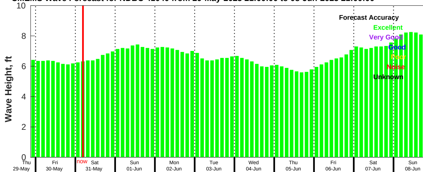
CMEMS Wave Forecast for NDBC 41040 from 29-May-2025 21:00:00 to 08-Jun-2025 21:00:00
