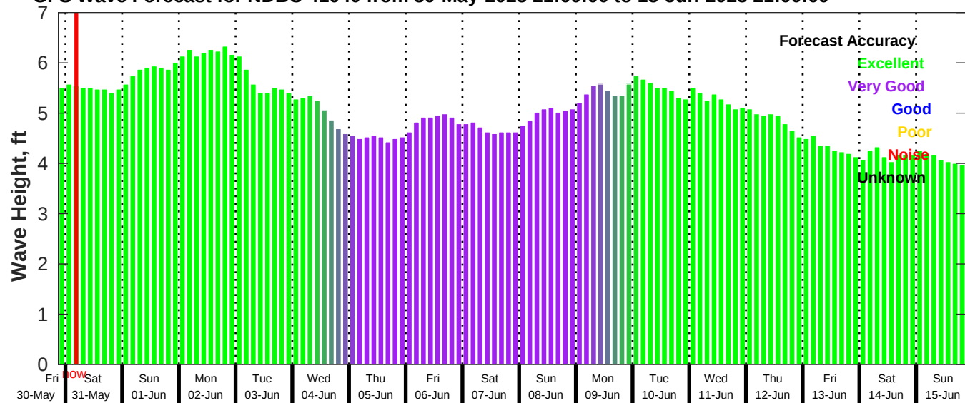
GFS Wave Forecast for NDBC 41040 from 30-May-2025 21:00:00 to 15-Jun-2025 21:00:00
