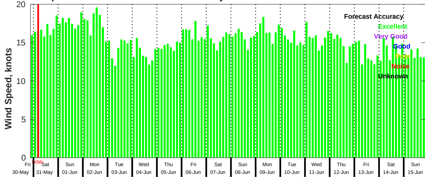
GFS Wind Speed Forecast for NDBC 41040 from 30-May-2025 21:00:00 to 15-Jun-2025 21:00:00
