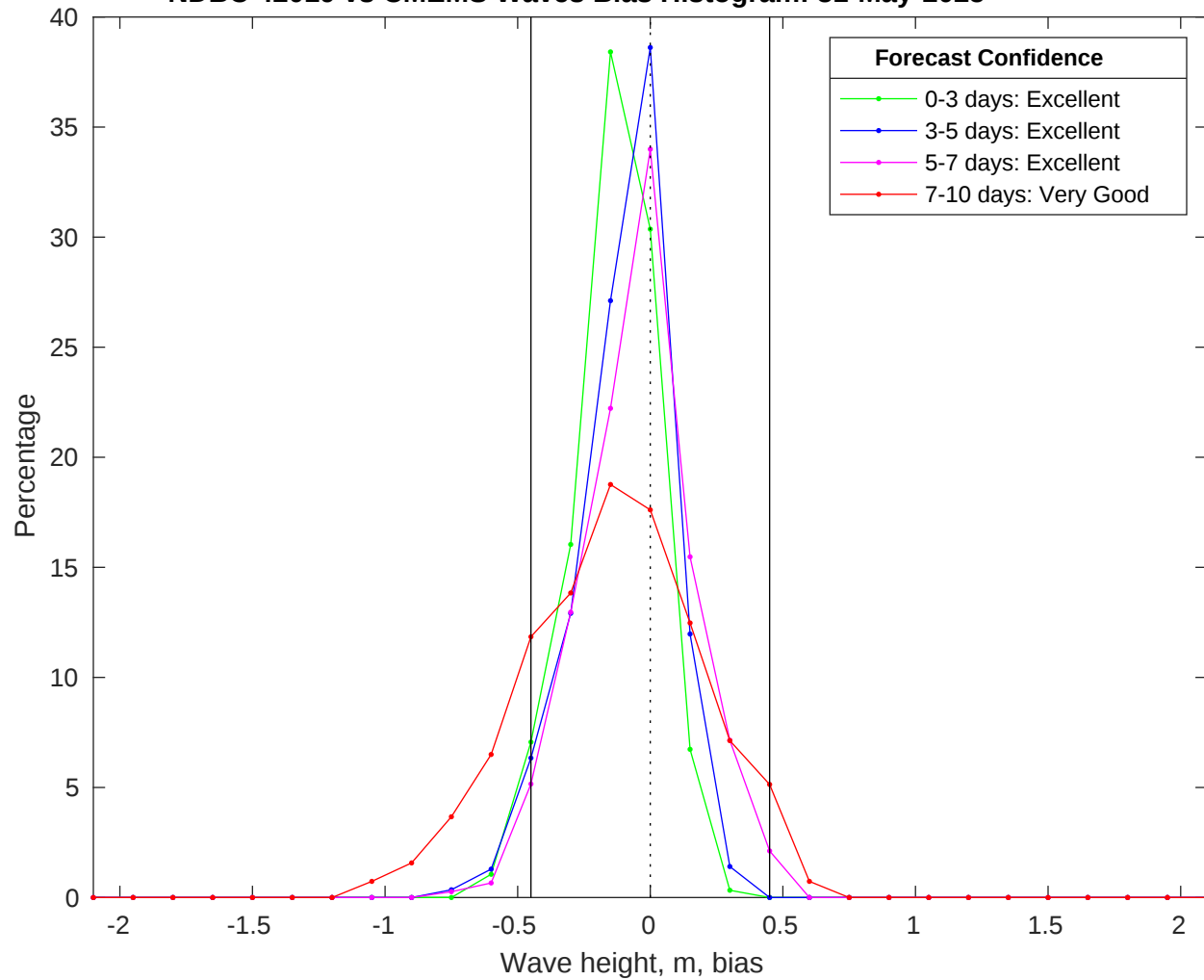
NDBC 42019 vs CMEMS Waves Bias Histogram: 31-May-2025
