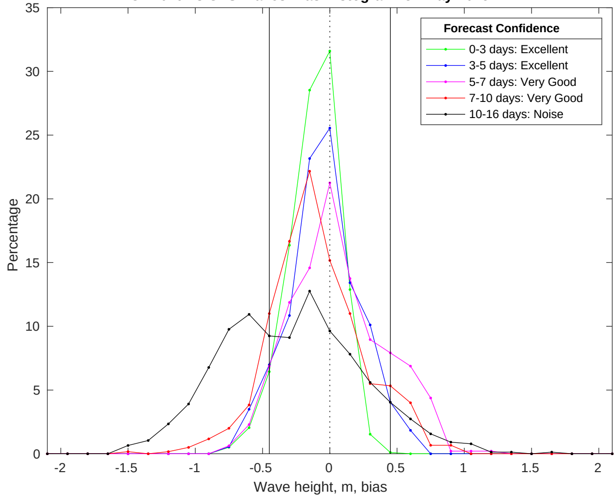
NDBC 42019 vs GFS Waves Bias Histogram: 31-May-2025
