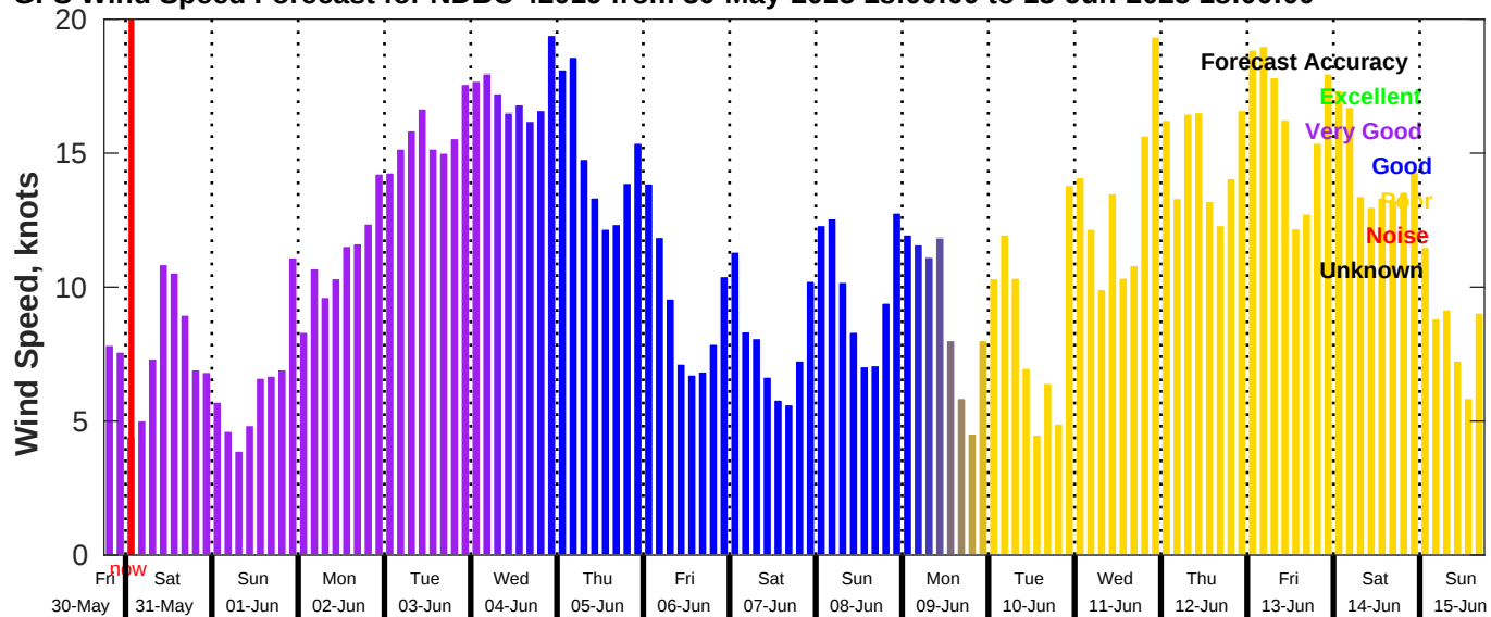
GFS Wind Speed Forecast for NDBC 42019 from 30-May-2025 18:00:00 to 15-Jun-2025 18:00:00
