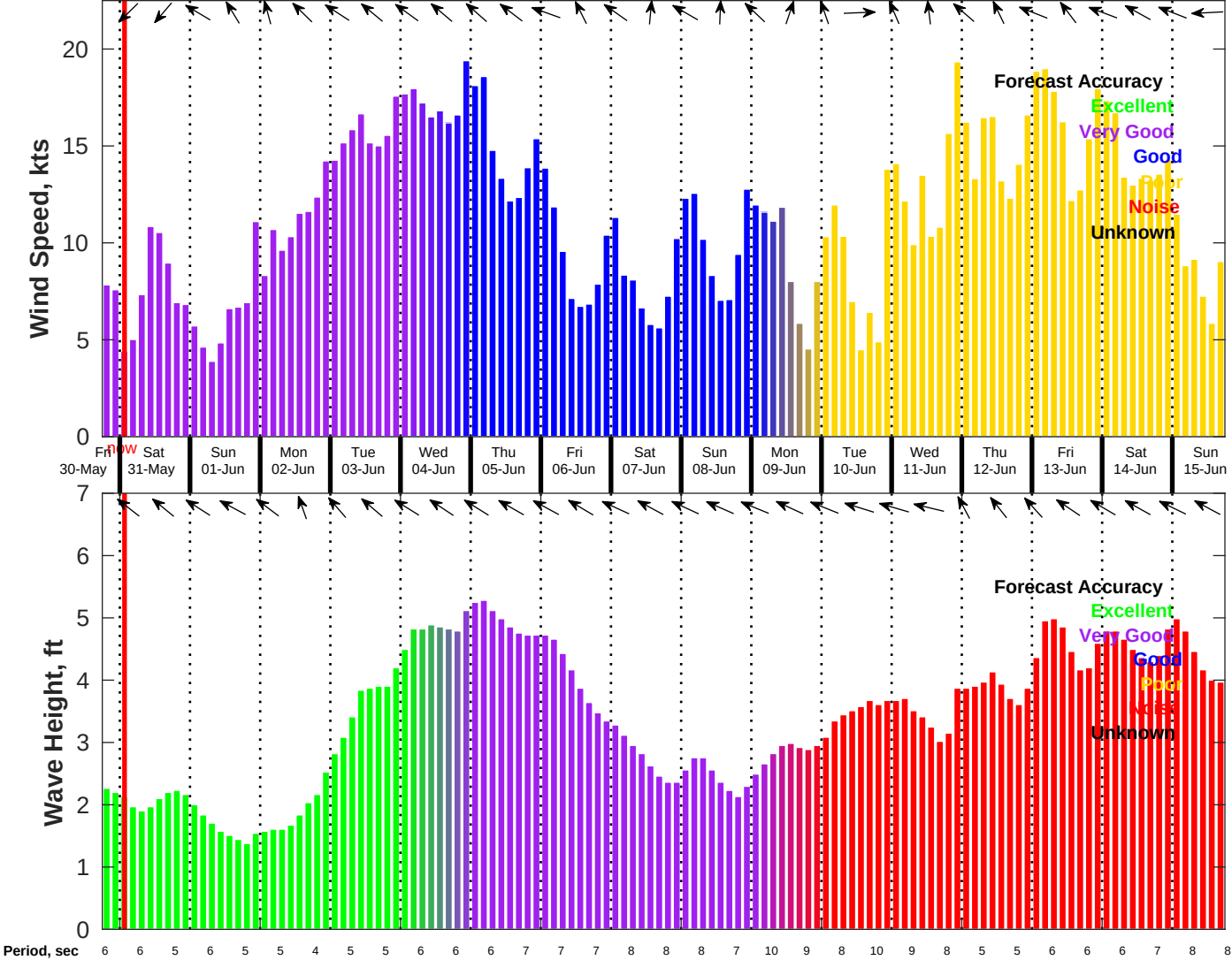
Wind & Wave Forecast for NDBC 42019 from 30-May-2025 18:00:00 to 15-Jun-2025 18:00:00
