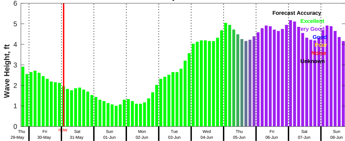
CMEMS Wave Forecast for NDBC 42020 from 29-May-2025 18:00:00 to 08-Jun-2025 18:00:00
