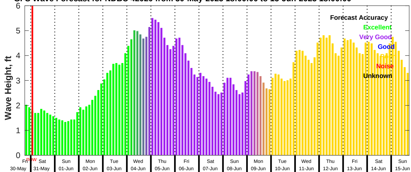
GFS Wave Forecast for NDBC 42020 from 30-May-2025 18:00:00 to 15-Jun-2025 18:00:00
