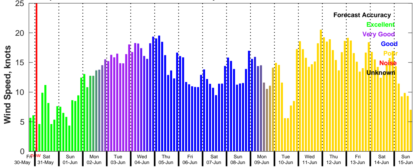
GFS Wind Speed Forecast for NDBC 42020 from 30-May-2025 18:00:00 to 15-Jun-2025 18:00:00
