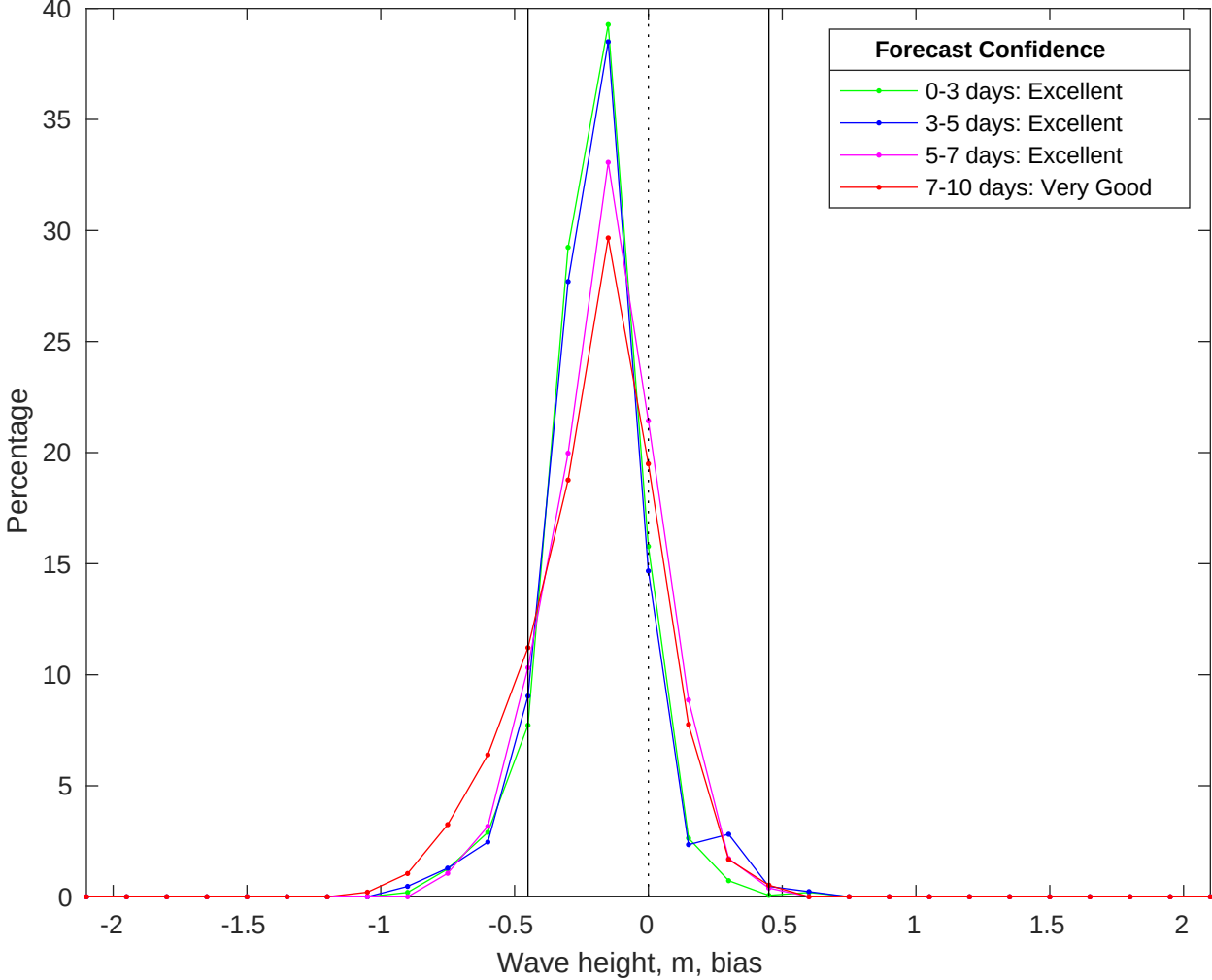
NDBC 42035 vs CMEMS Waves Bias Histogram: 31-May-2025
