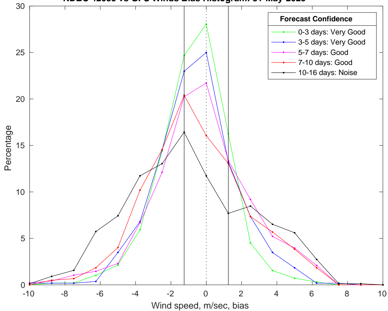
NDBC 42035 vs GFS Winds Bias Histogram: 31-May-2025
