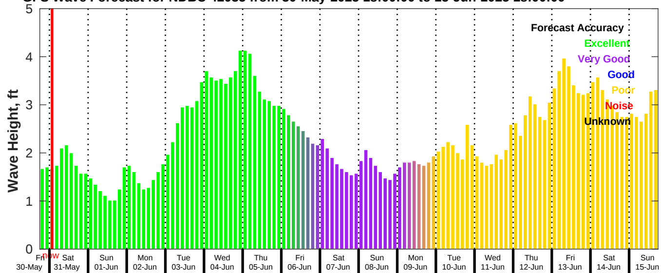
GFS Wave Forecast for NDBC 42035 from 30-May-2025 18:00:00 to 15-Jun-2025 18:00:00
