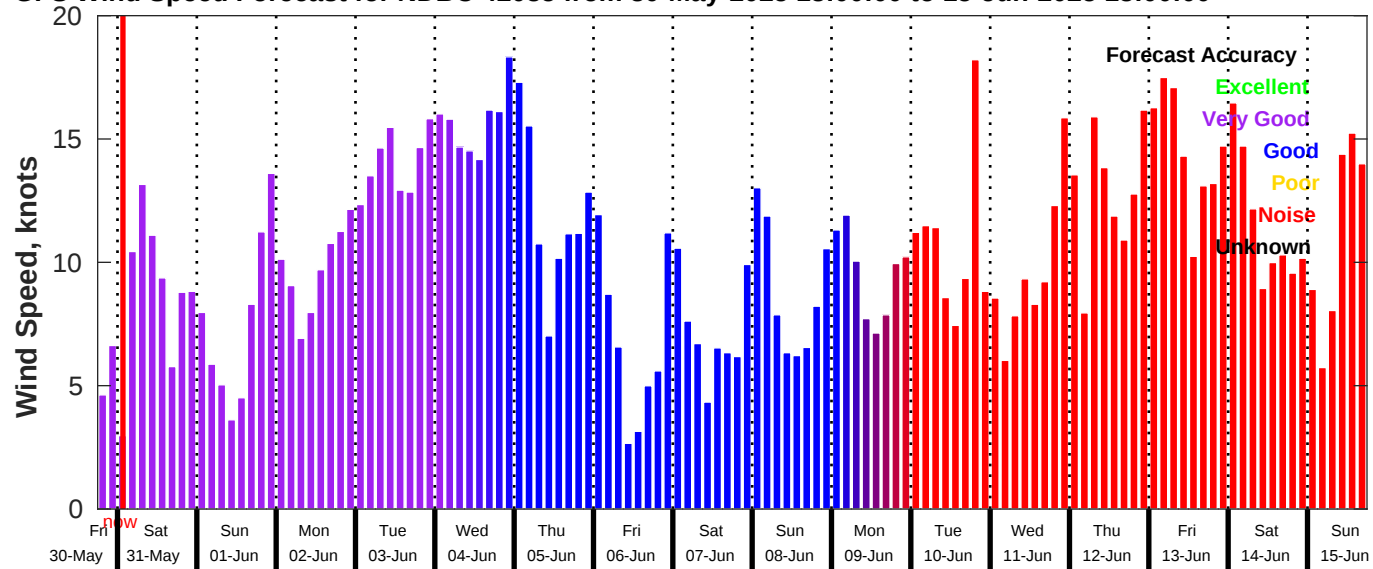
GFS Wind Speed Forecast for NDBC 42035 from 30-May-2025 18:00:00 to 15-Jun-2025 18:00:00
