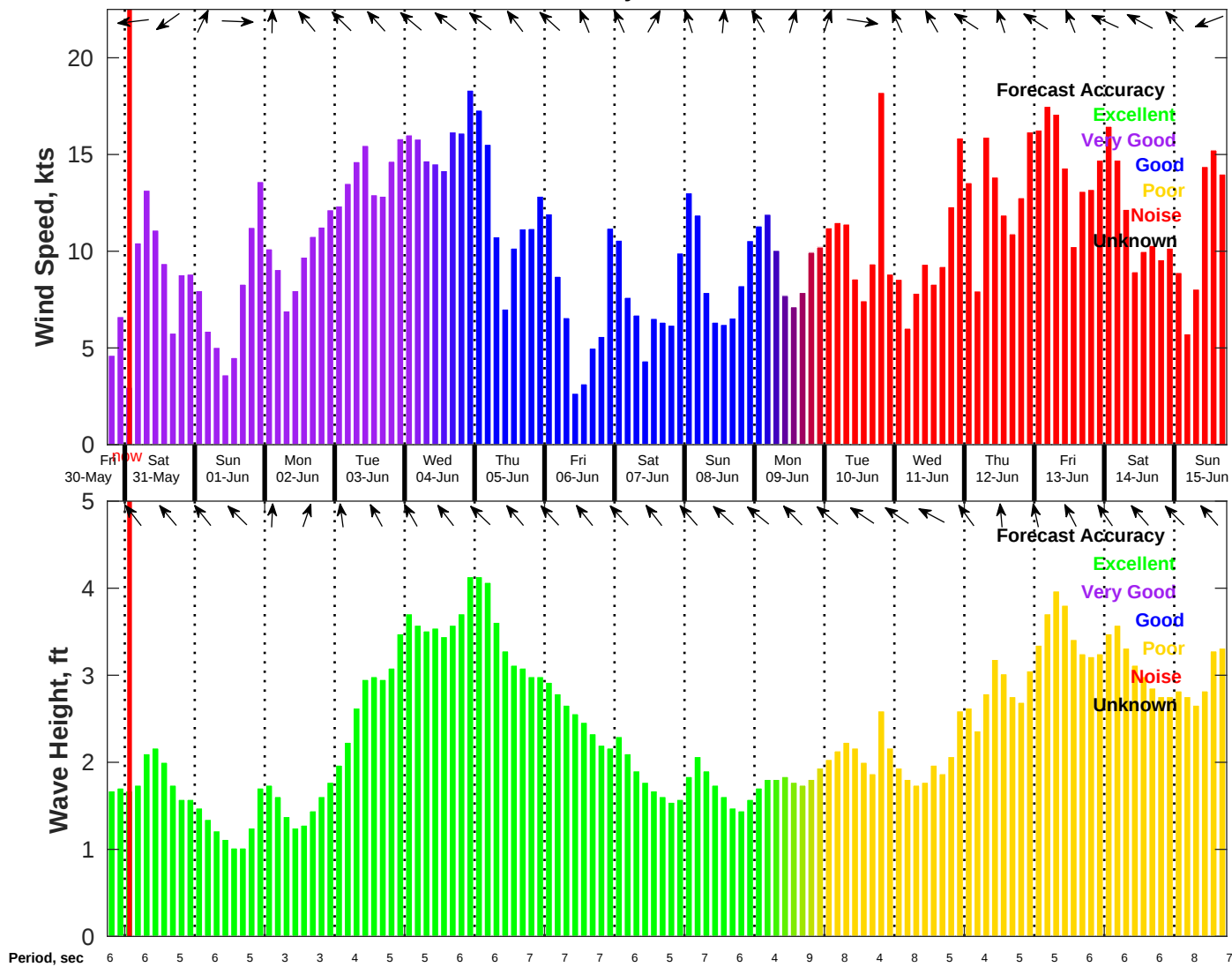
Wind & Wave Forecast for NDBC 42035 from 30-May-2025 18:00:00 to 15-Jun-2025 18:00:00
