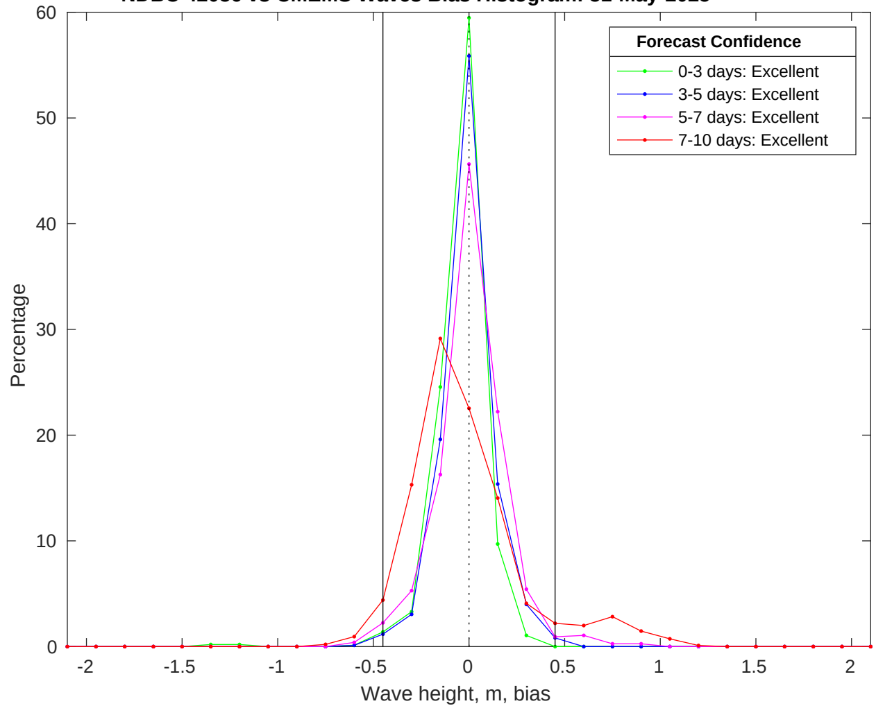
NDBC 42036 vs CMEMS Waves Bias Histogram: 31-May-2025
