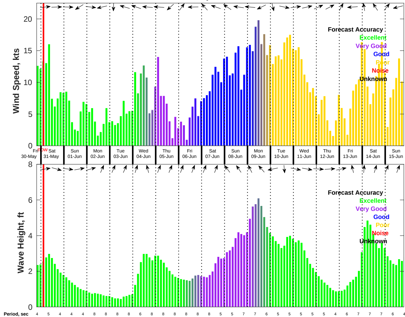
Wind & Wave Forecast for NDBC 42036 from 30-May-2025 19:00:00 to 15-Jun-2025 19:00:00
