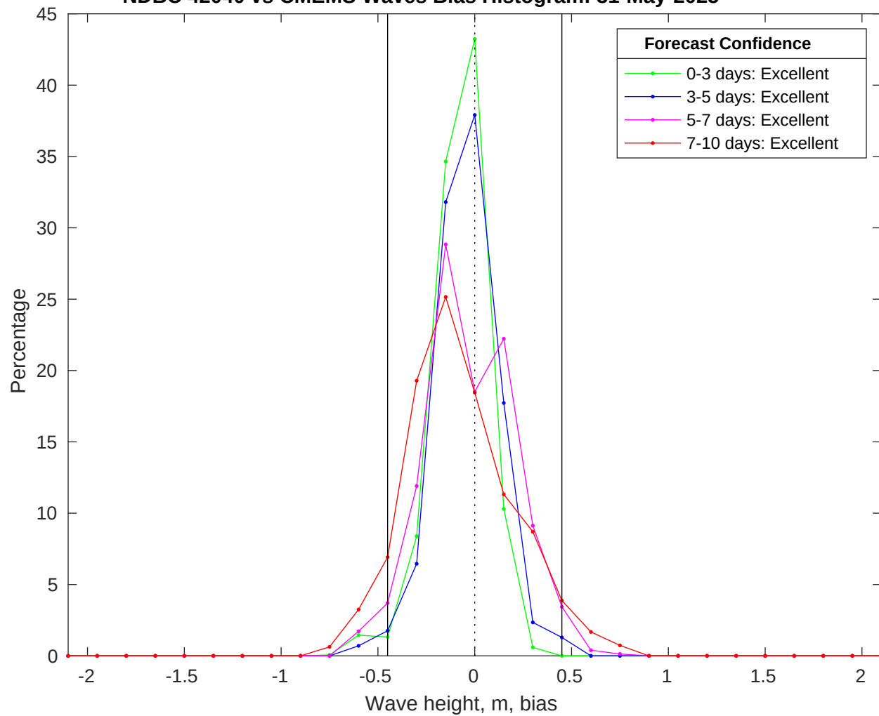
NDBC 42040 vs CMEMS Waves Bias Histogram: 31-May-2025
