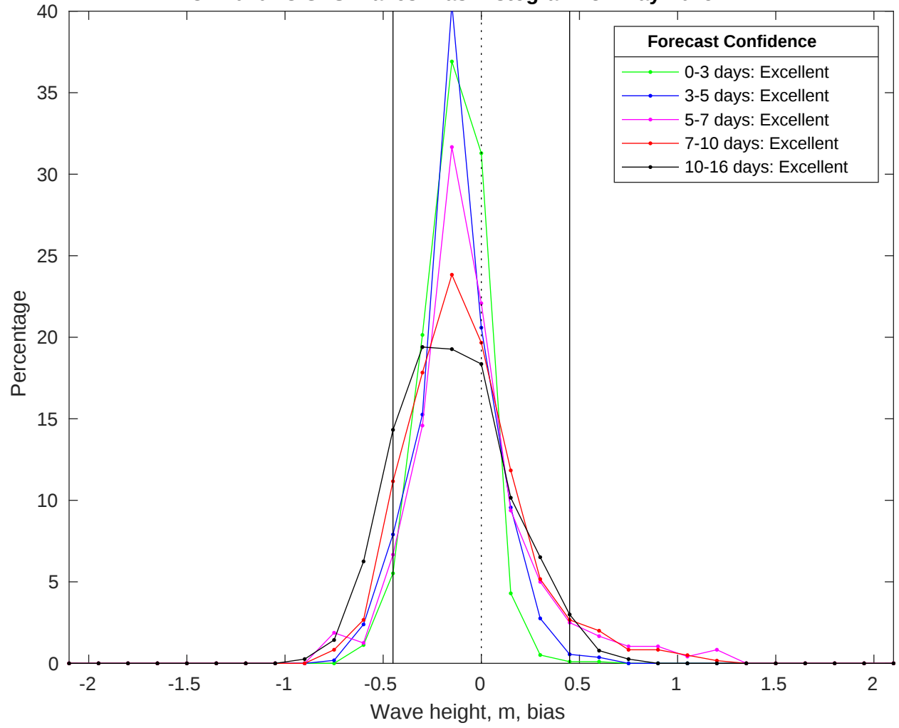
NDBC 42040 vs GFS Waves Bias Histogram: 31-May-2025
