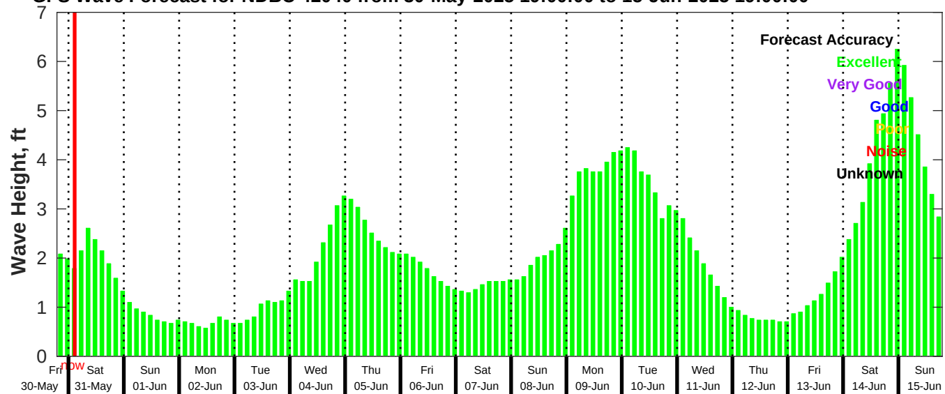
GFS Wave Forecast for NDBC 42040 from 30-May-2025 19:00:00 to 15-Jun-2025 19:00:00
