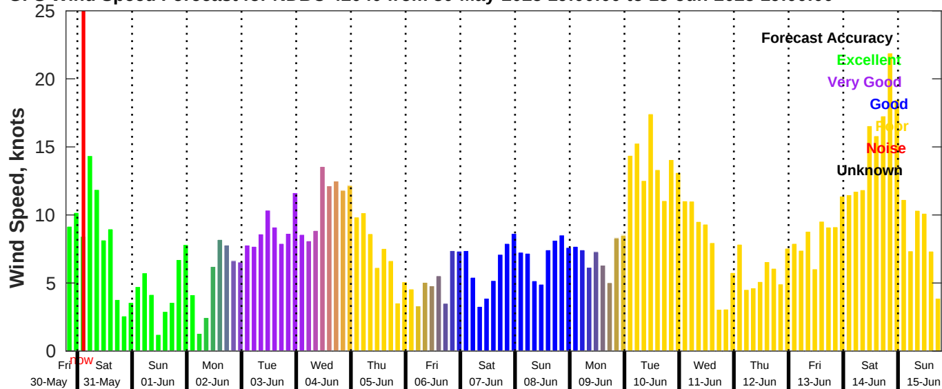
GFS Wind Speed Forecast for NDBC 42040 from 30-May-2025 19:00:00 to 15-Jun-2025 19:00:00
