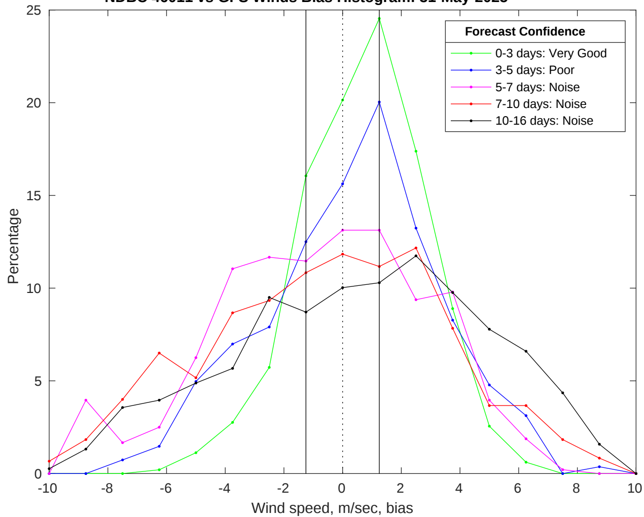
NDBC 46011 vs GFS Winds Bias Histogram: 31-May-2025
